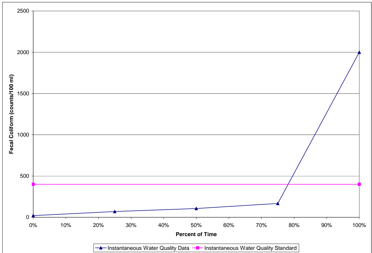
Figure 8. 10% Test Curve for Station A0390006, Summer 2008
