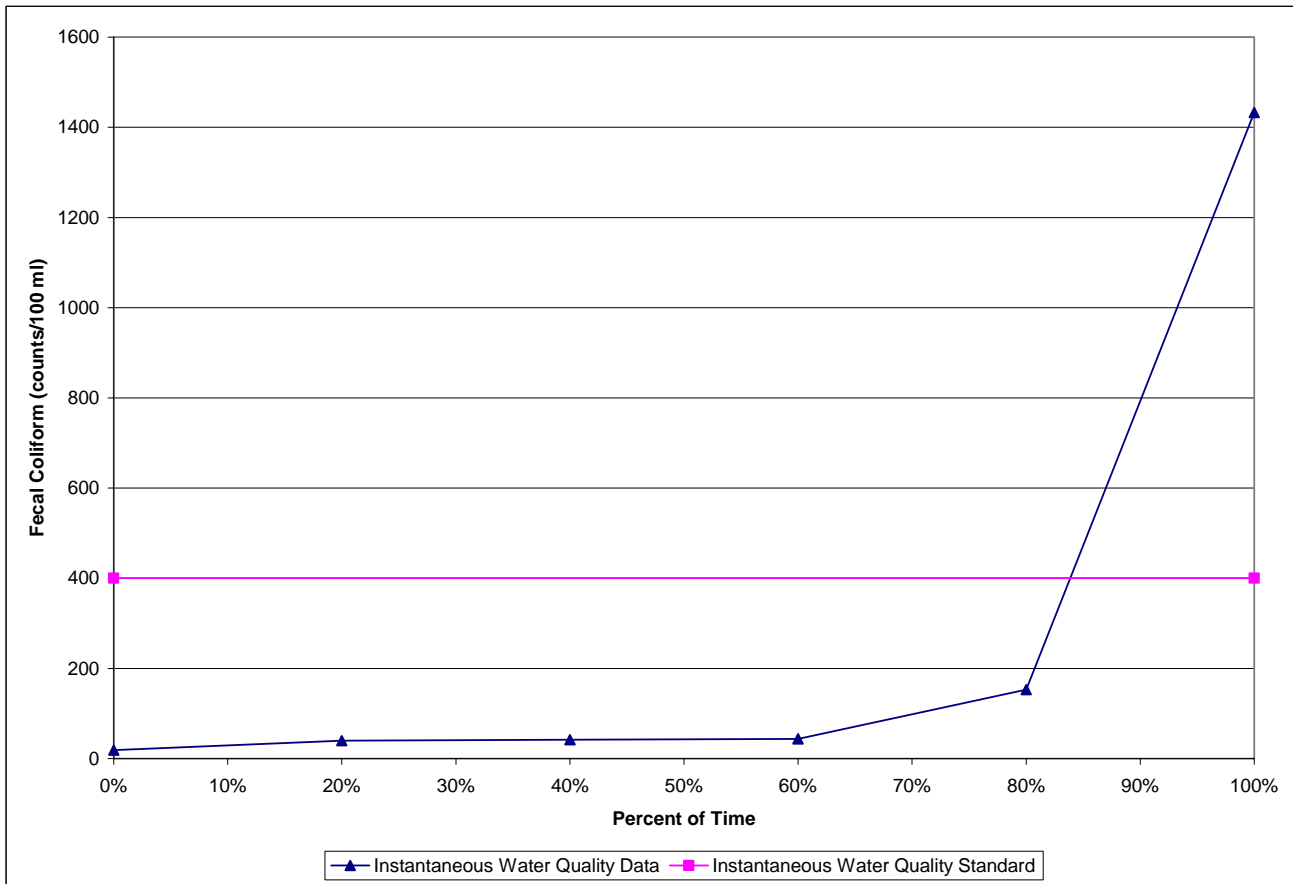
Figure 7. 10% Test Curve for Station A1110009, Winter 2009
