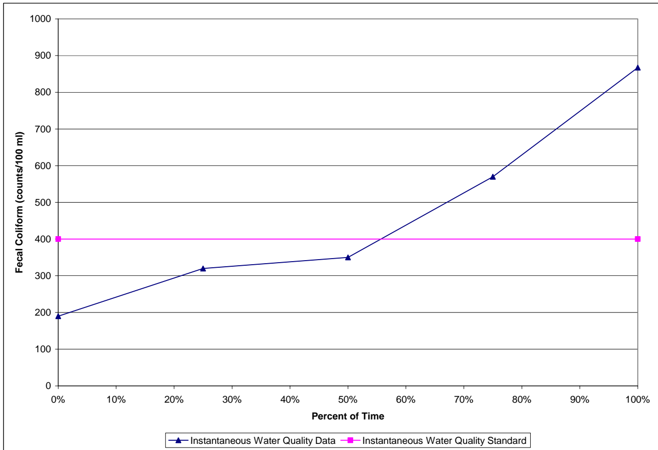
Figure 9. 10% Test Curve for Station A0390006, Winter 2008
