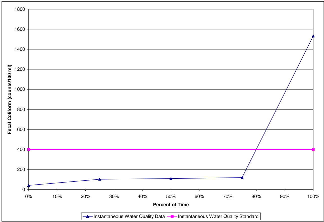
Figure 6. 10% Test Curve for Station A1110009, Summer 2008
